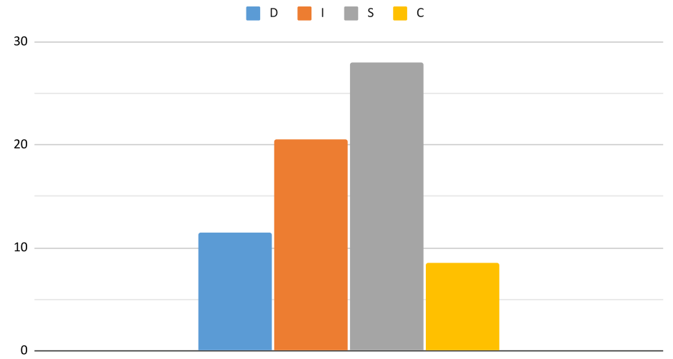
Natural Style
